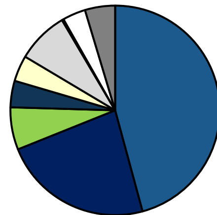
Karyotypes
